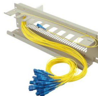
Implementation Example (Chassis and Modules)
