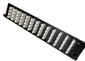
104-fiber DLC Adapter Panel (2U, Transparent)
